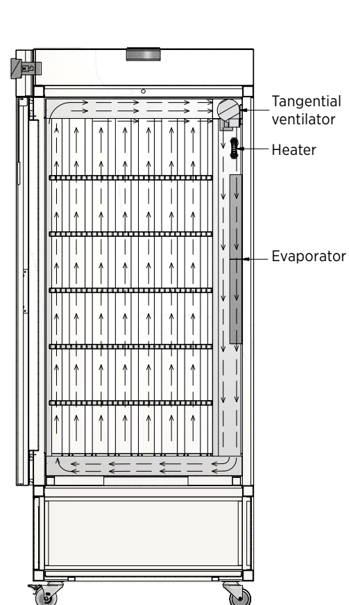
Fig. 1 Air circulation
